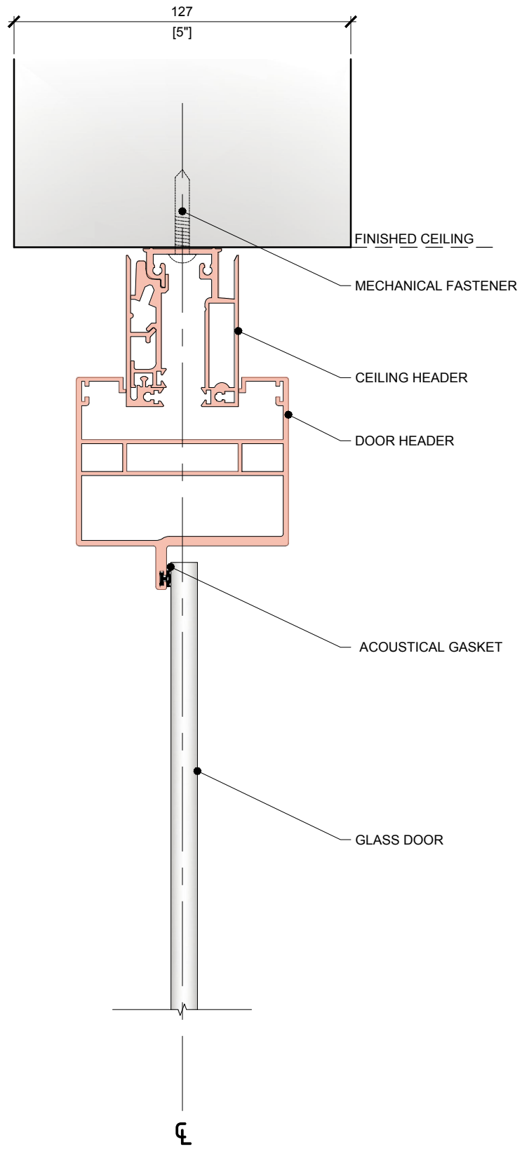
01 DWEL: GLASS HINGED DOOR - FULL HEIGHT D1 1:2
