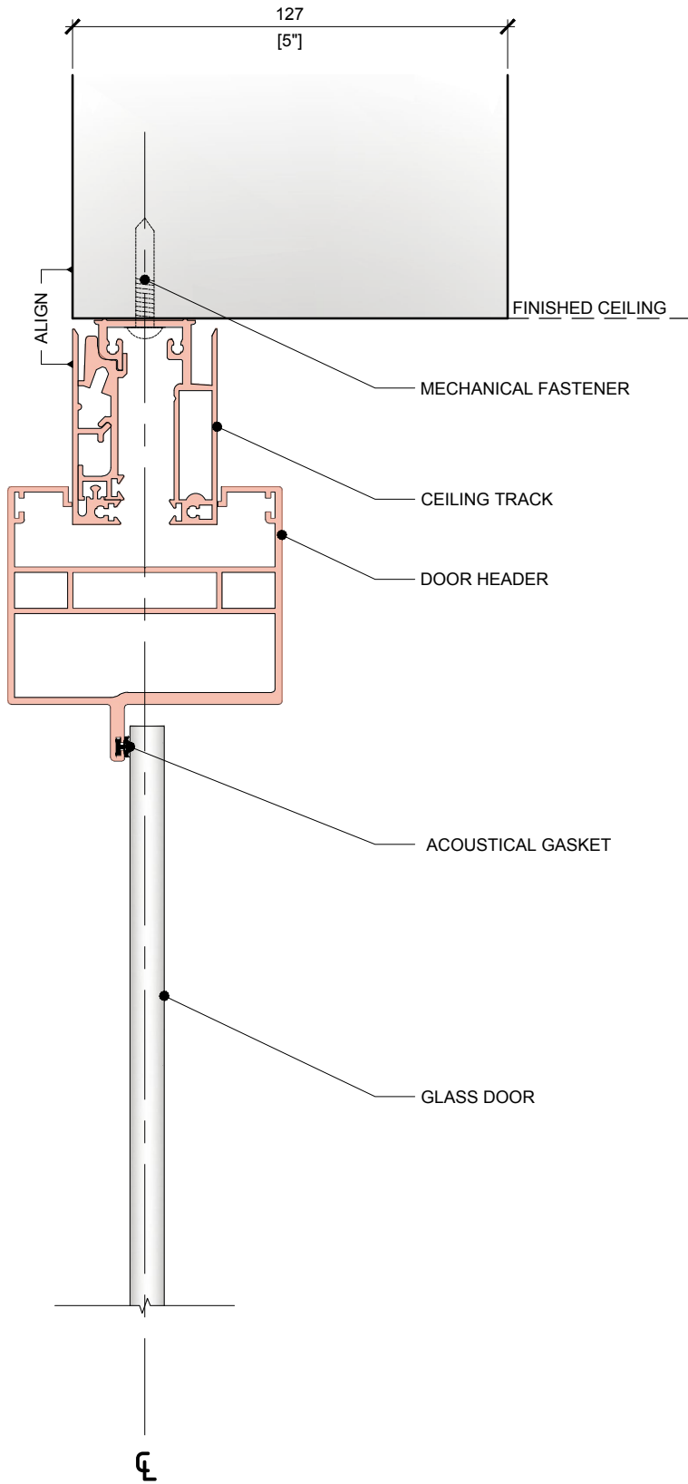
01 DWEL: GLASS HINGED DOOR - FULL HEIGHT D17 1:2
