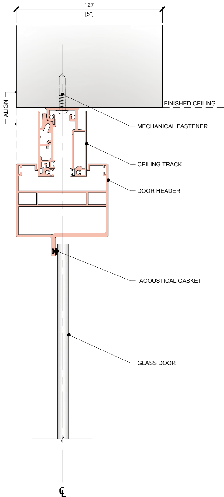
01 DWEL: GLASS HINGED DOOR - FULL HEIGHT D23 1:2
