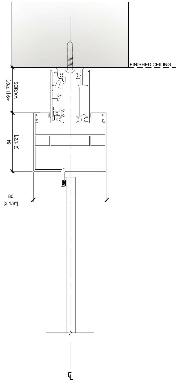
01 DM1 DWEL: GLASS HINGED DOOR - FULL HEIGHT - DIM 1:2
