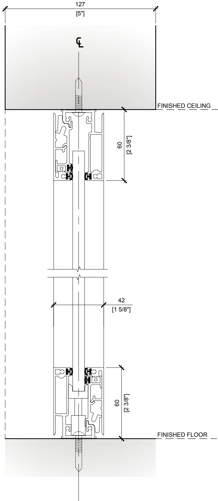
01 DWEL: GLAZING FRONT SECTION - DIM DM16 1:2
