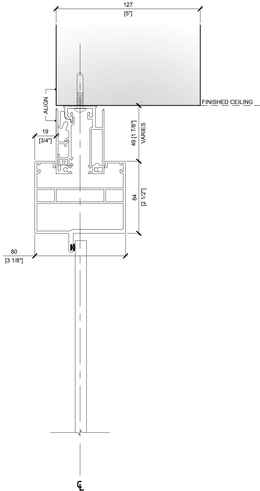
01 DWEL: GLASS HINGED DOOR - FULL HEIGHT - DIM DM17 1:2
