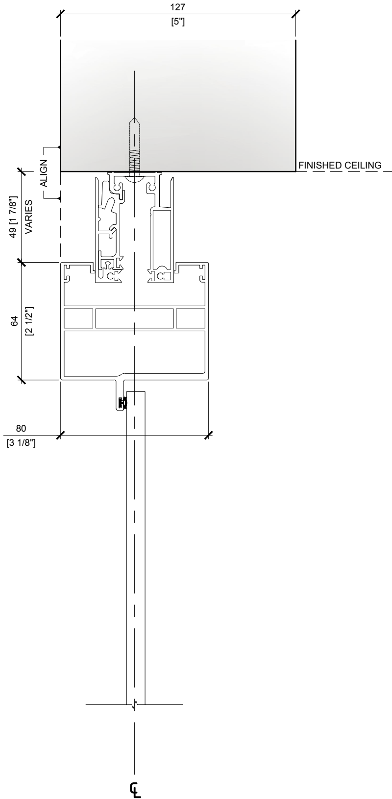
01 DWEL: GLASS HINGED DOOR - FULL HEIGHT - DIM DM23 1:2
