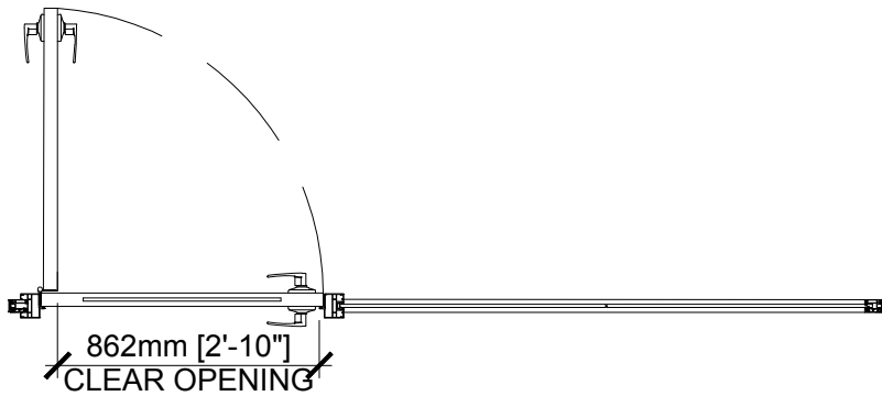
01 DWEL: WOOD DOOR WITH GLASS INSERT - FULL HEIGHT E111 NTS
