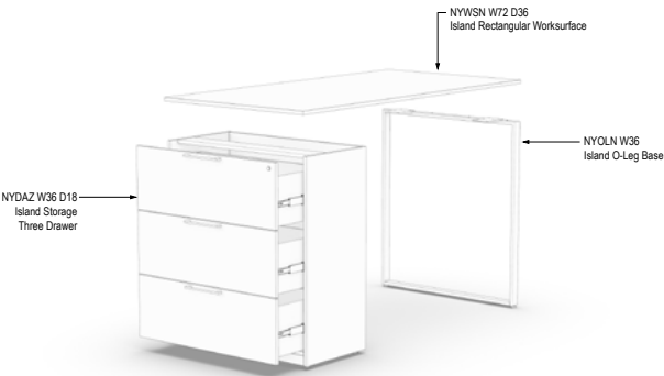
Island Table Exploded View
