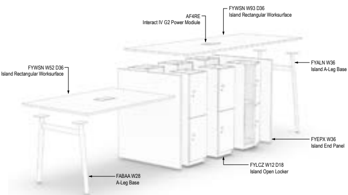
Island Table Exploded View
