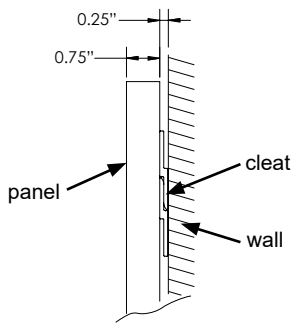
Total depth from wall is 1.00"
