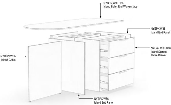
Island Table Exploded View
