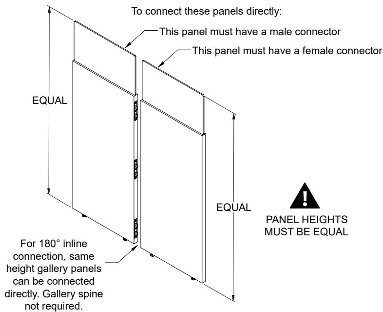
180° Direct Connection
