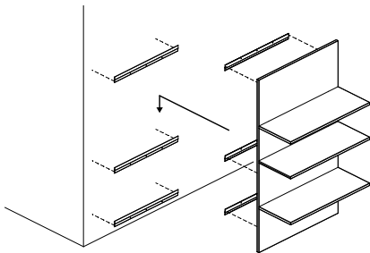
Wall panels drop into cleat
