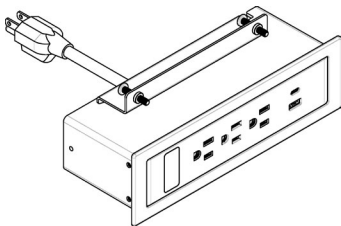
TRIO FLUSH MOUNT
