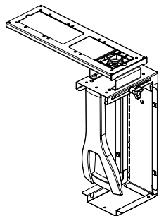
FULL SIZE SLIDE & SWIVEL
