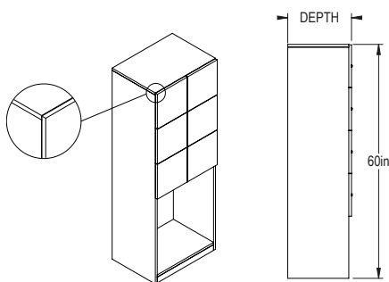
CONFIG: 24" WIDE
