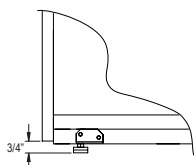
Full Front or 1" Kick (Z)
